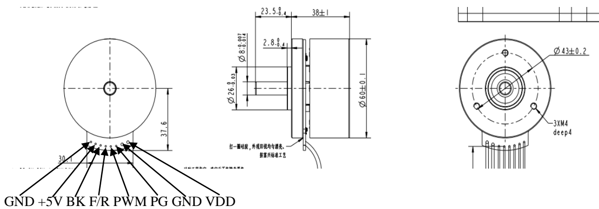
FIG. 1 Mechanical dimensions
