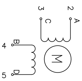
Wiring Diagram (接线图)
